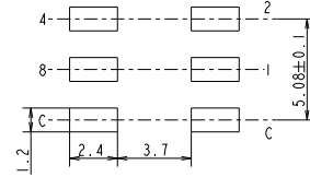
P. C. B DIMENSION
