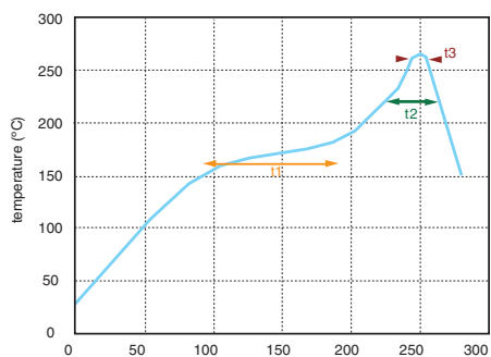
SMT reflow soldering profile of reference
