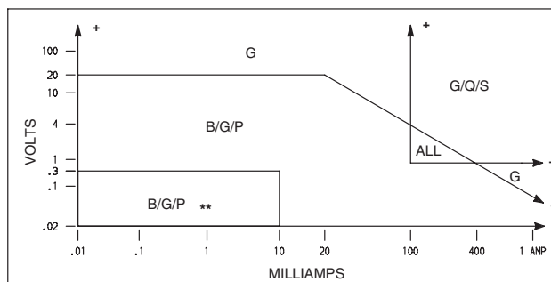
RECOMMENDED CONTACT MATERIALS VS. VOLTAGE AND CURRENT
